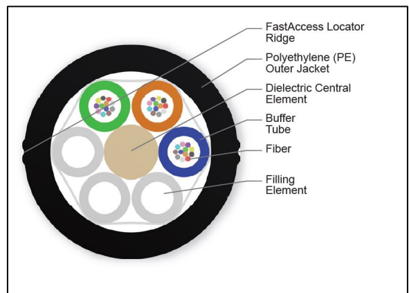
Fiber SenSys Part Number 600-83121
